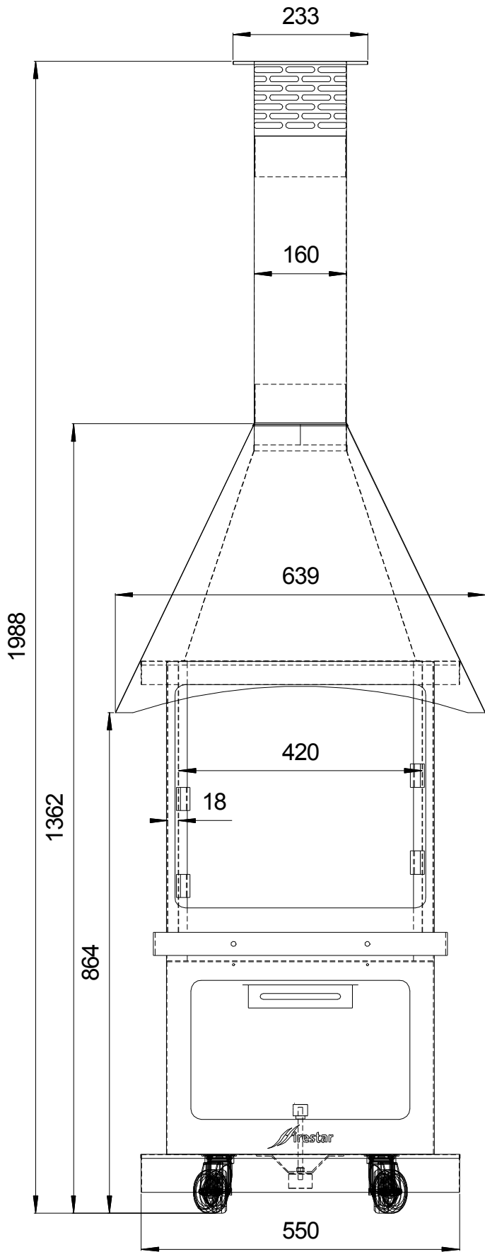
firestar DN 550
