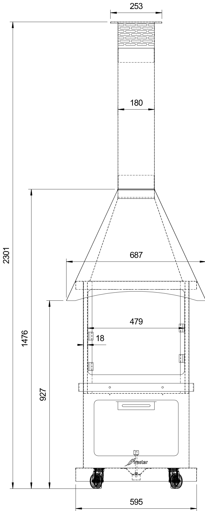
firestar DN 650 Swing 3. Generation
