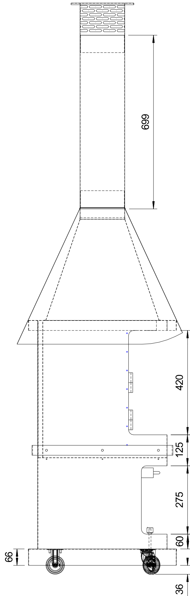
firestar DN 650 Swing 3. Generation
