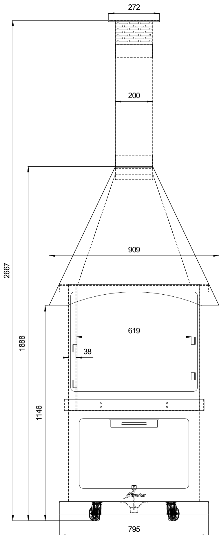
firestar DN 800 Swing / GLAS 3. Generation
